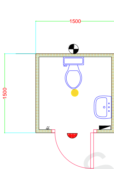
FLOOR PLAN
