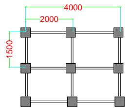
FOUNDATION PLAN PRECAST BLOCK SIZE 40 X 40 X 40
