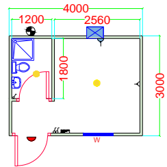
FLOOR PLAN
