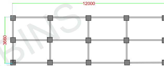
FOUNDATION PLAN PRECAST BLOCK 40 X 40 X 40
