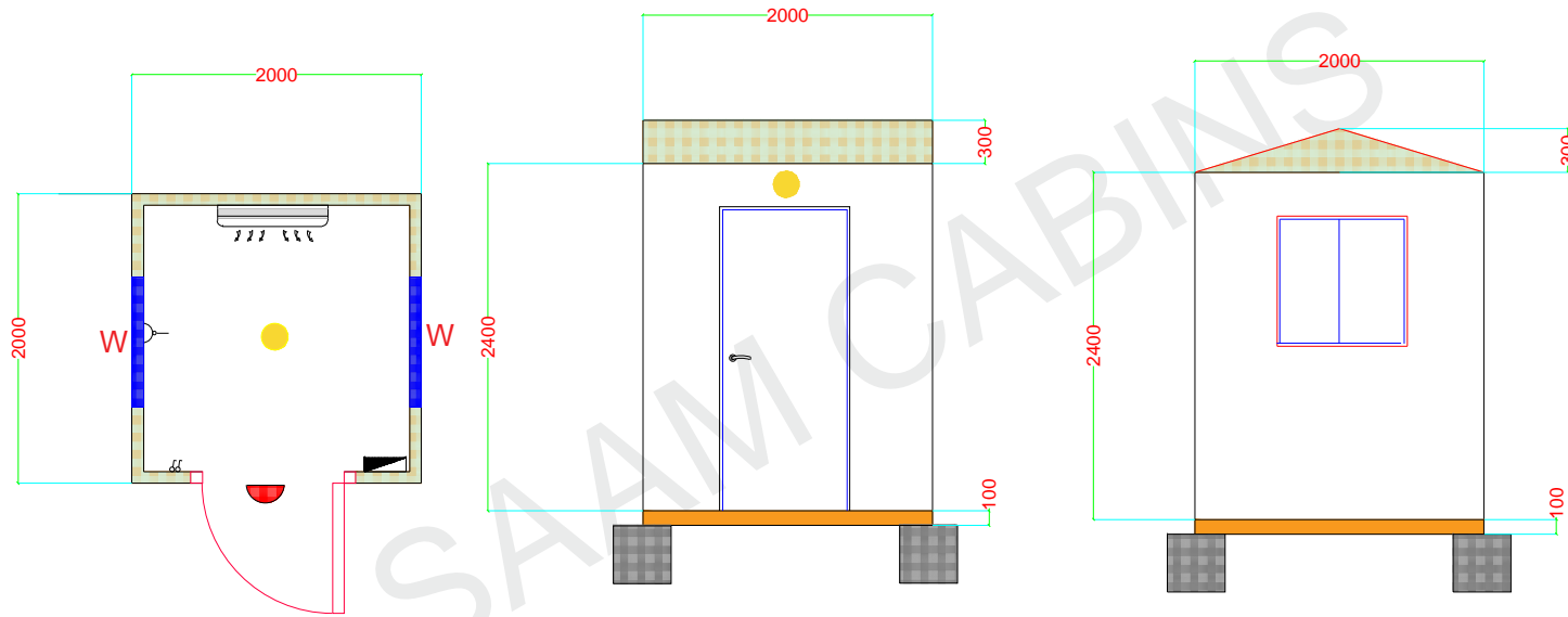
SIDE ELEVATION
