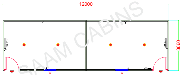
FLOOR PLAN
