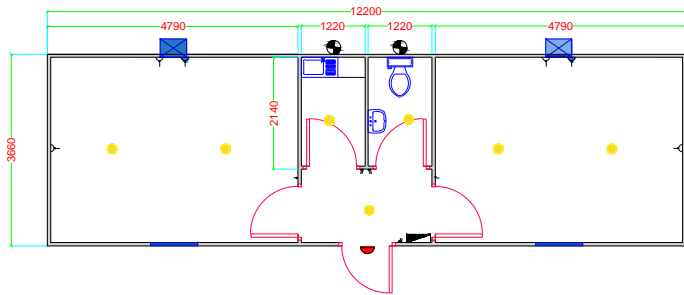
FLOOR PLAN
