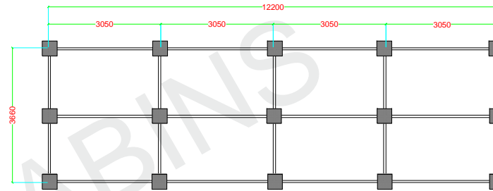
FOUNDATION PLAN PRECAST BLOCK SIZE 40 X 40 X 40
